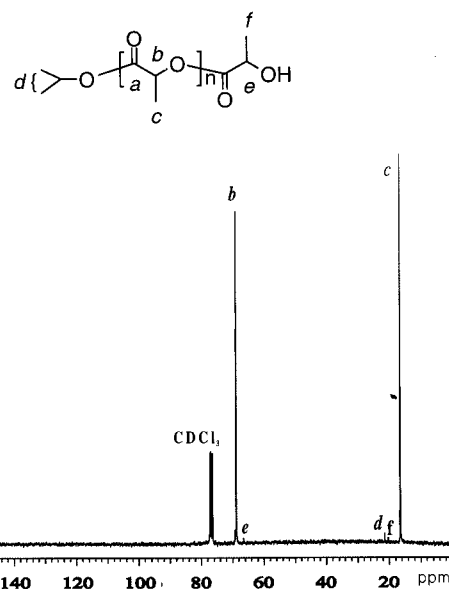
Figure 7. The 75.26 MHz ^{13}\text{C} NMR spectrum ( \text{CDCl}_3 ) of poly-(L-LA) obtained with 2-PrOH- \text{Ca}[\text{N}(\text{SiMe}_3)_2]_2(\text{THF})_2 (molar ratio: 2/1) (entry 4, Table 1).
